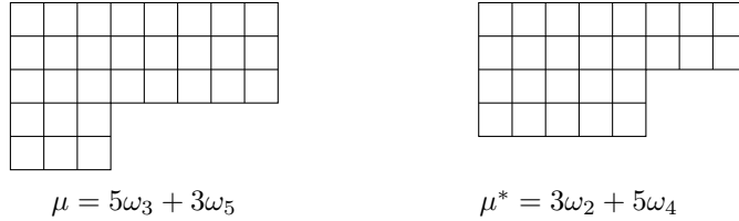
FIGURE 3. In this example, with n = 7 , \mu corresponds to the partition [8, 8, 8, 3, 3] and \mu^* corresponds to the partition [8, 8, 5, 5] .
