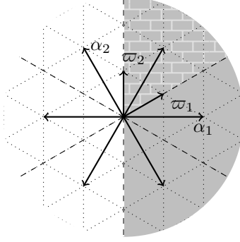
FIGURE 1. Roots and fundamental weights for \mathrm{SL}(3, \mathbb{C}) . The positive Weyl chamber of \mathrm{GL}(2, \mathbb{C}) is light gray and it contains the positive Weyl chamber of \mathrm{SL}(3, \mathbb{C}) which is filled with bricks.
