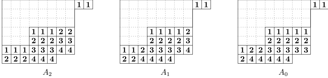
FIGURE 4. In this example we have n = 7 , \mu, \mu^* as in Figure 3 and k = 2 . There are three configurations of \mathbf{1} 's leading to three Littlewood-Richardson skew tableaux.
